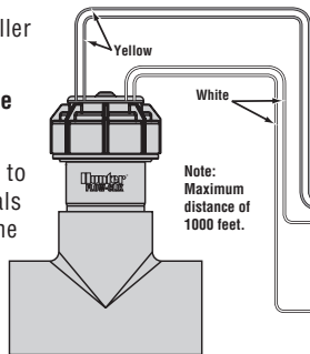
Flow-Clik IMMS Sensor
